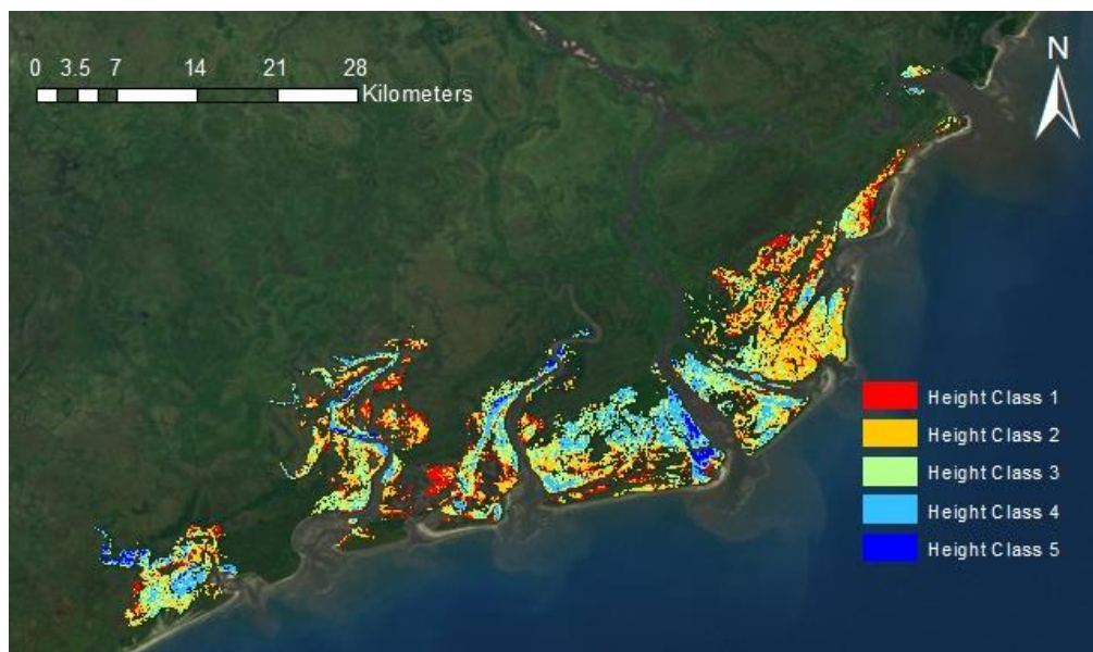
Figure 5.2. Distribution of mangrove canopy height class in the Zambezi River Delta. Canopy height data obtained from Fatoyinbo and Simard (2013). The associated height range for each class is shown in Table 5.1.
