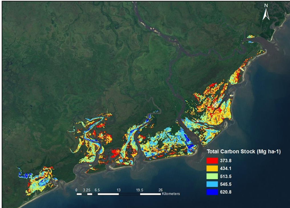
Figure 6.10. Spatial distribution of mangrove ecosystem carbon stocks in the Zambezi River Delta.
