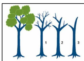
Figure 5.10. Decay classes used to categorize standing dead trees (Kauffman and Donato 2012).
