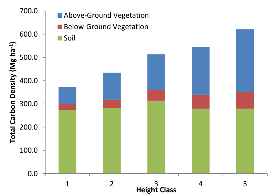
Figure 6.9. Contributions of biomass and soil carbon pools to ecosystem carbon density within height classes. Values represent the mean of each height class.
