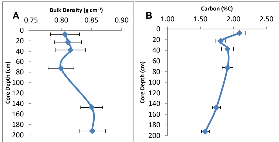
Figure 6.8. Mean soil bulk density (A) and carbon concentration (B) with depth; error bars represent the standard error.
