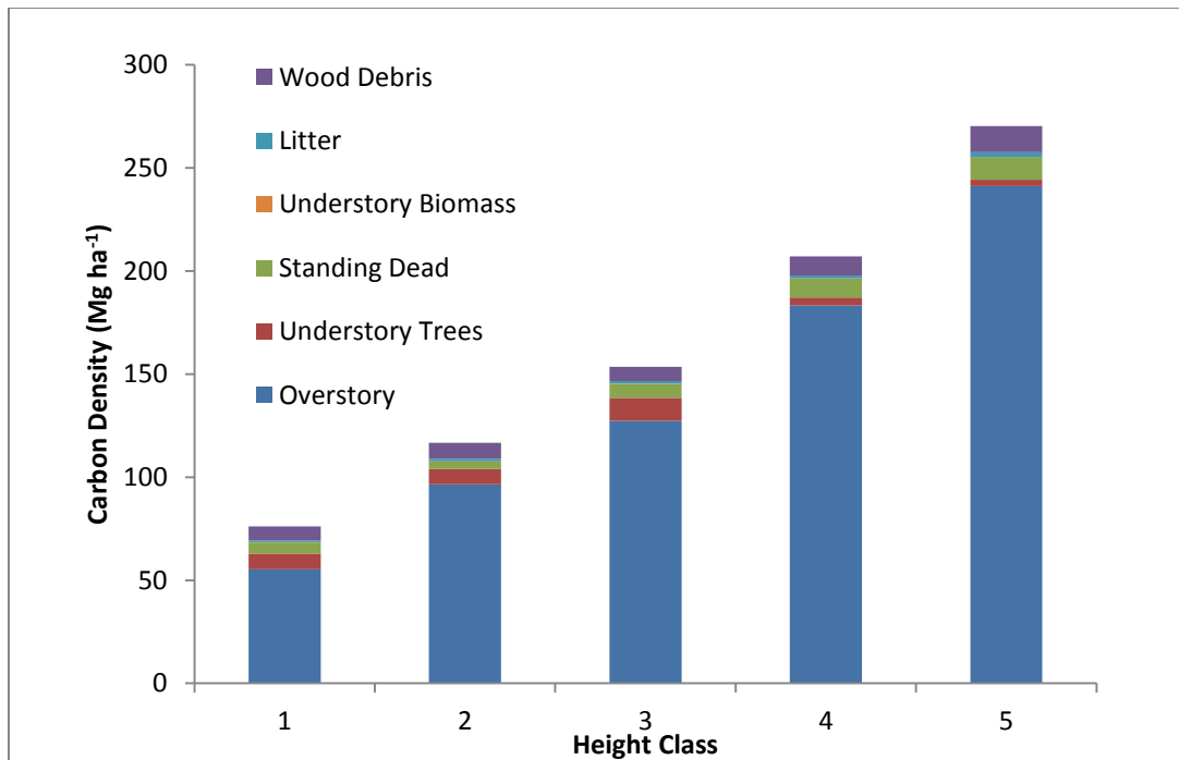
Figure 6.6. Contributions of biomass components to above-ground carbon density; the values represent the average within height classes.
