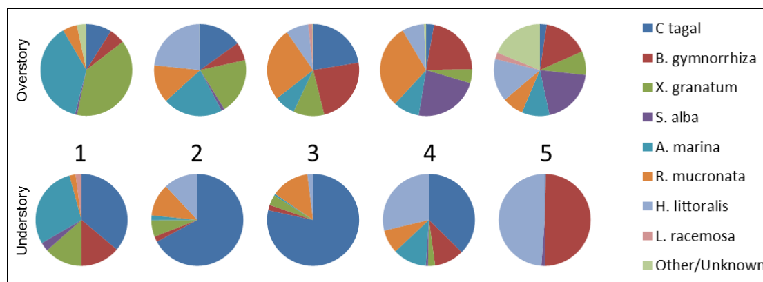
Figure 6.3. Proportional contribution of each species to above-ground biomass carbon density for overstory trees (top) and understory trees (bottom).
