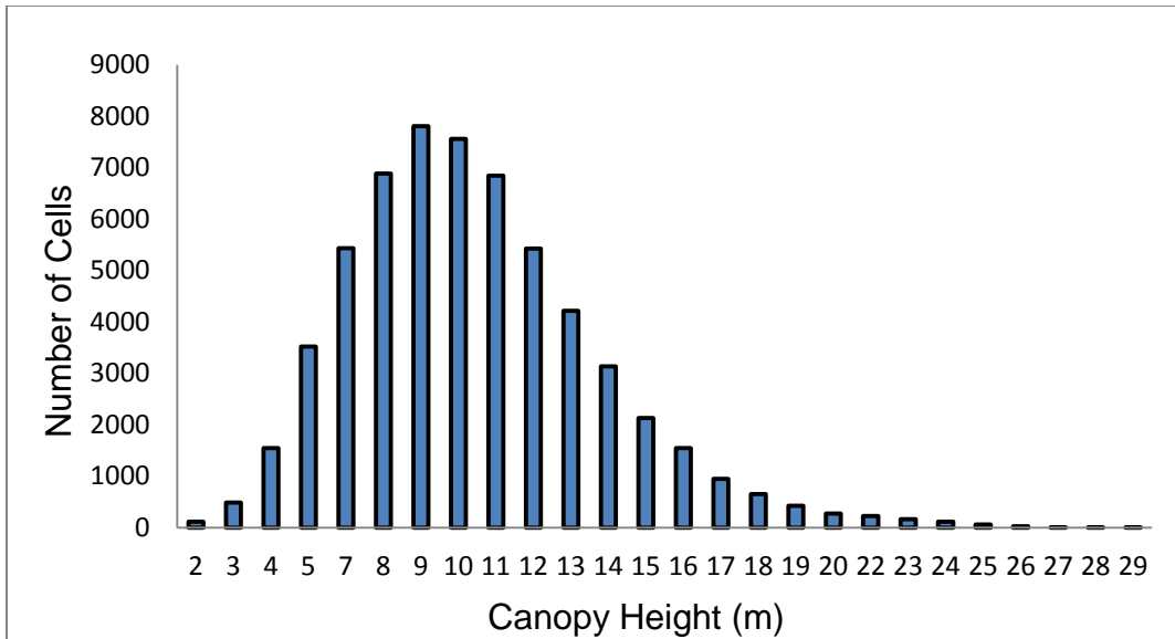
Figure 5.3. Distribution of pixel (cells) canopy height values, as determined by analysis of SRTM data (data from T.E. Fatoyinbo, NASA).
