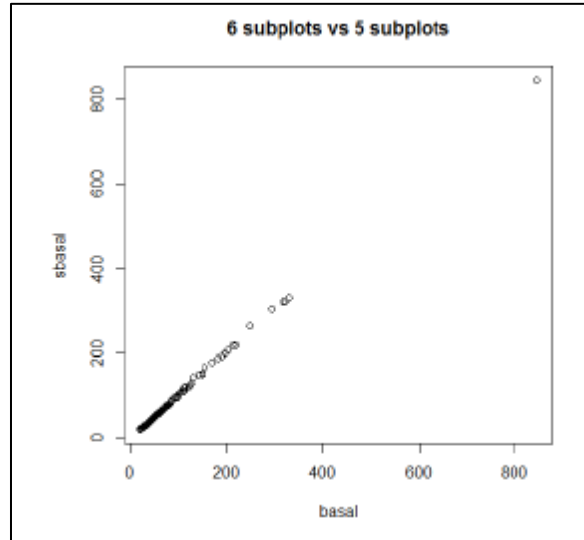
Figure 5.6. Plot showing differences of empirical distributions of estimates based on 5 and 6 subplots (Tang, et al. 2013).
